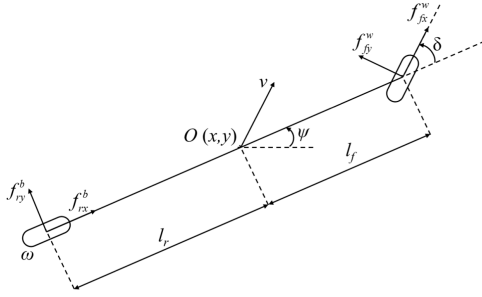
Fig. 4. Bicycle model [72].
